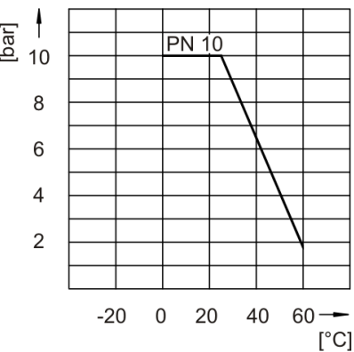
Pressure – Temperature diagram - PVDF
