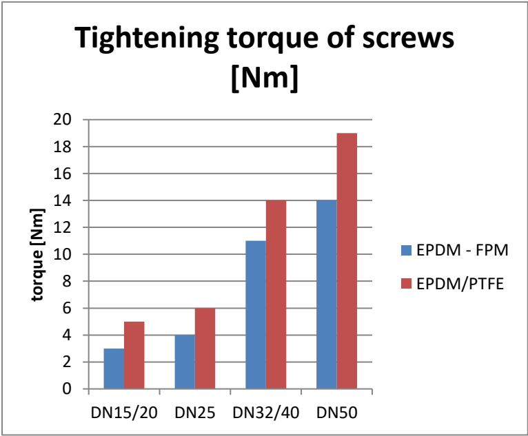
Tightening torque of screws
