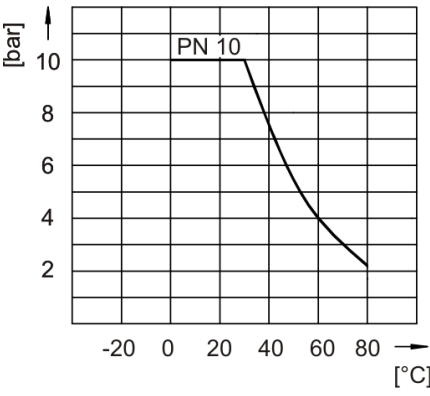
Pressure – Temperature diagram - PP
