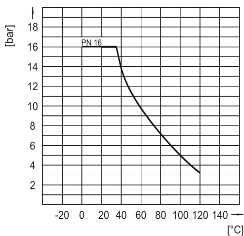
Pressure-temperature-diagram – PVDF
