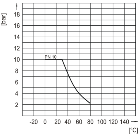
Pressure-Temperature-Diagram – PP
