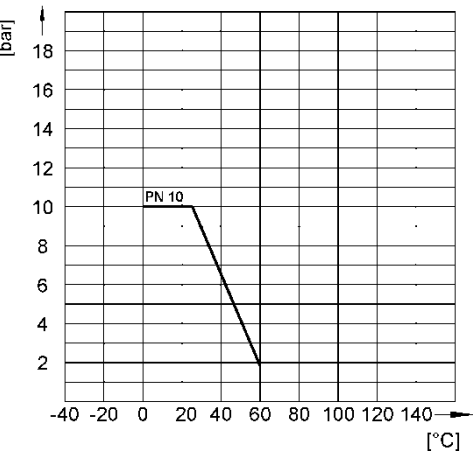
Pressure-Temperature-Diagram – PVC-U
