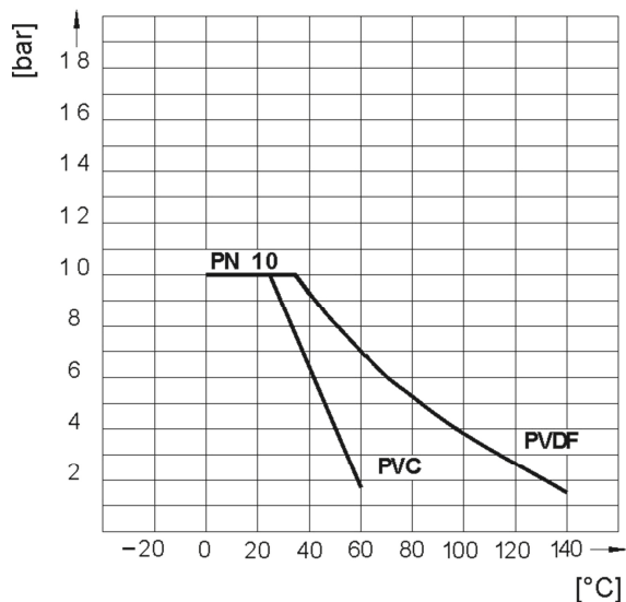
Pressure-temperature-diagram
